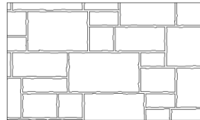
PERM_LAFITT50 Random Ashlar Bond with 50% large stones
