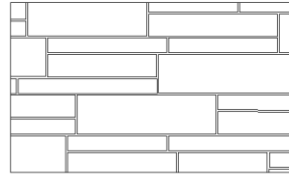
PERM_LEXA_C Random Ashlar Bond with 33% large stones
