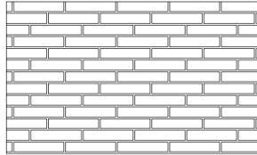
PERM_MELVILLE_NORMAN_B2 Modified running Bond Pattern
